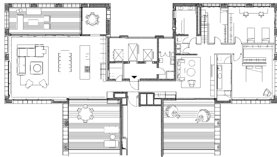
PLOT PLAN
